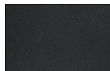
DARK GREY
